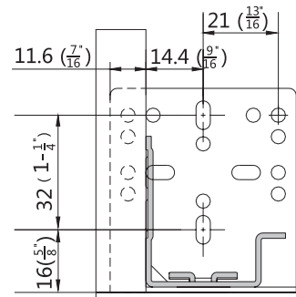
Metal rear mounting bracket 7800-BRKT
