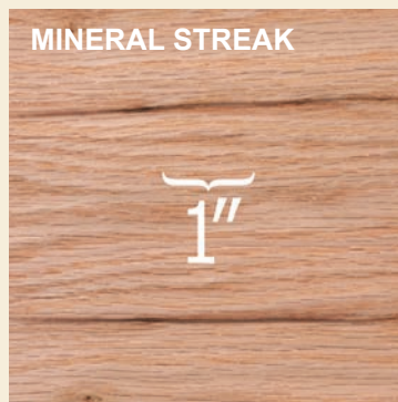
MINERAL STREAK
