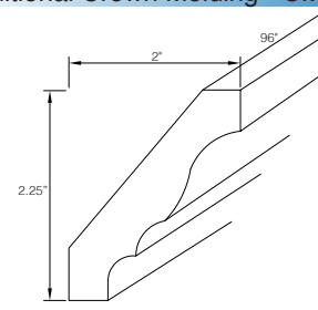
Traditional Crown Molding - CM8
