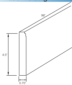
Furniture Base Molding - FBM8
