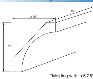
Cove Crown Molding - COM8
